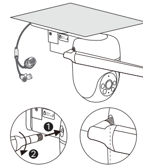
SMA Connector
