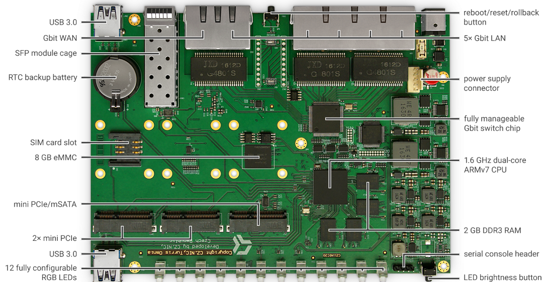
Turris Omnia: motherboard components
