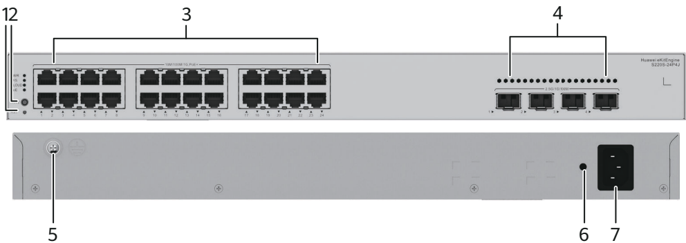
Figure 4-16 S220S-24P4J appearance
