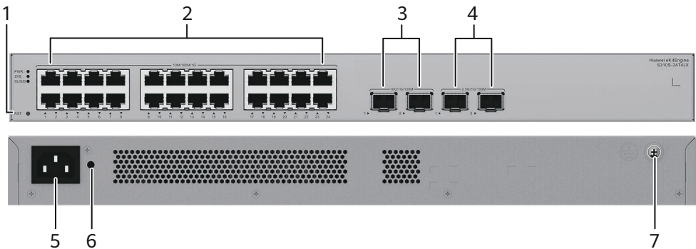
Figure 4-36 S310S-24T4JX appearance
