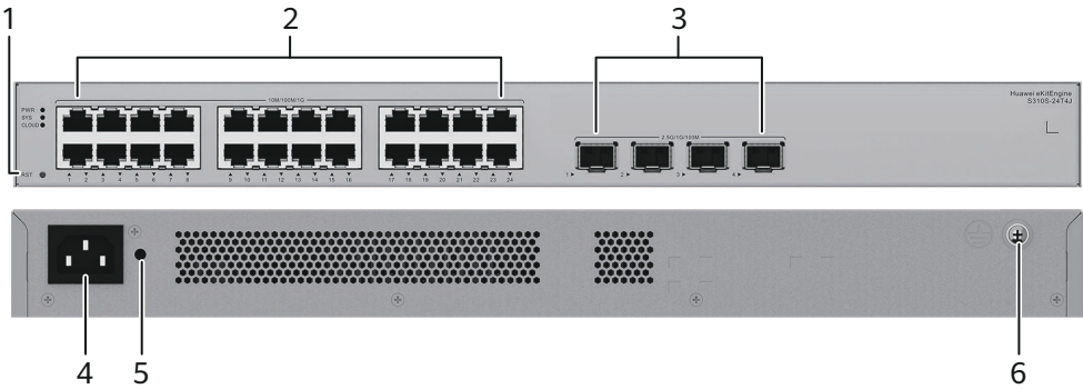
Figure 4-34 S310S-24T4J appearance
