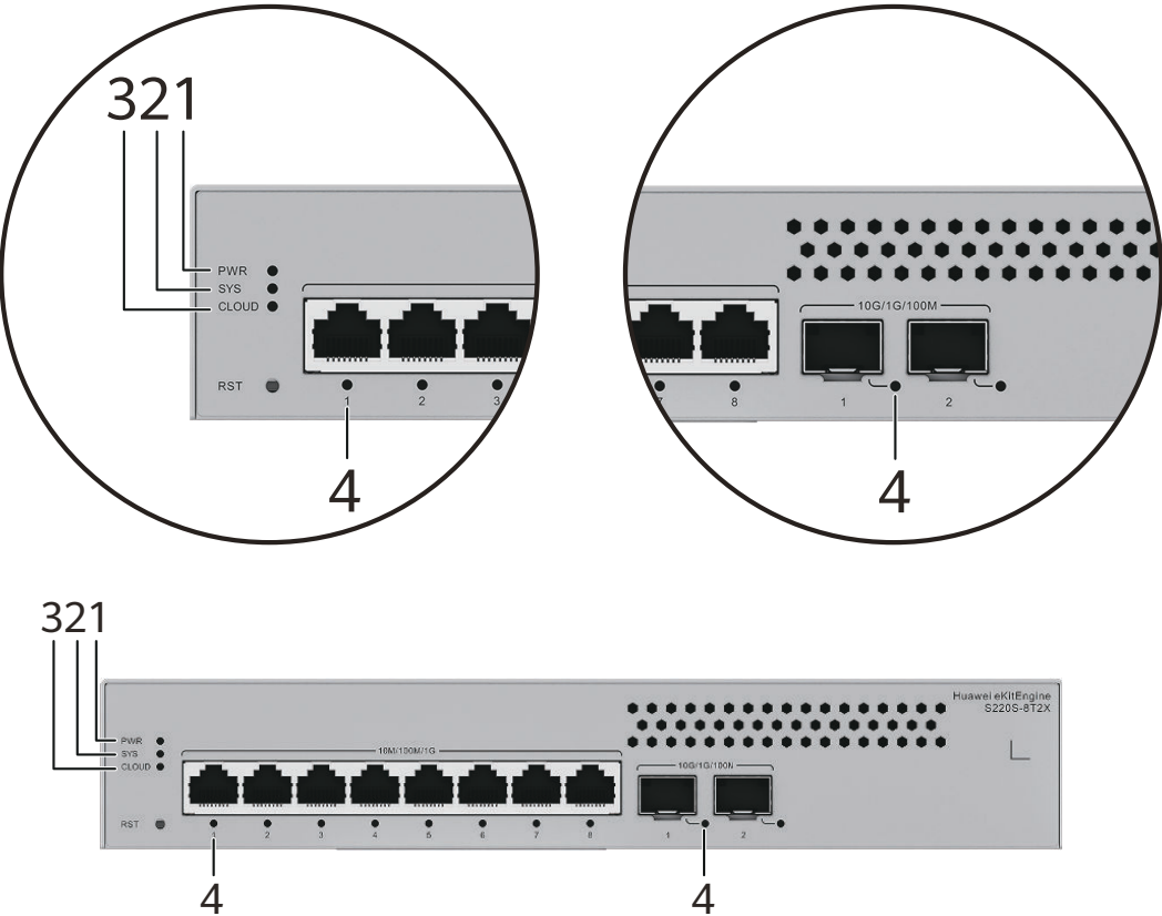
Figure 4-3 Indicators on the Switch
