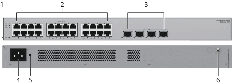
Figure 4-12 S220S-24T4J appearance
