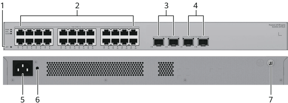
Figure 4-14 S220S-24T4JX appearance
