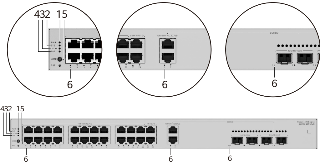
Figure 4-11 Indicators on the Switch
