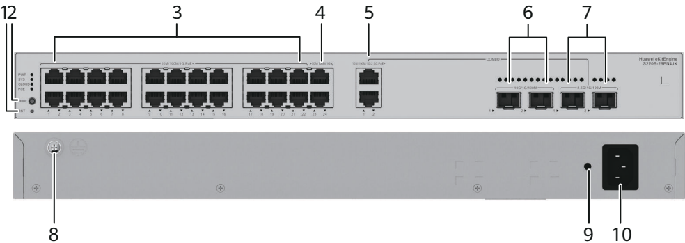
Figure 4-22 S220S-26PN4JX appearance
