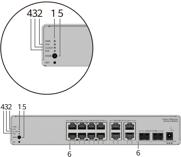
Figure 4-31 Indicators on the Switch
