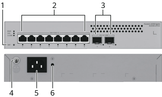
Figure 4-4 S220S-8T2X appearance
