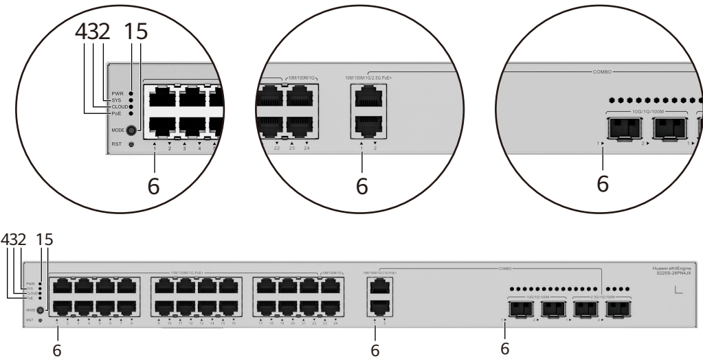
Figure 4-7 Indicators on the Switch
