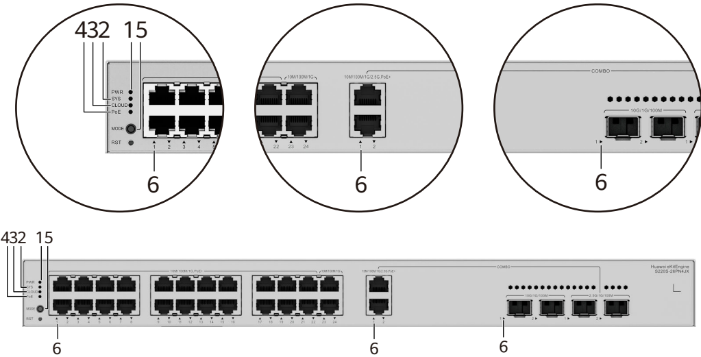
Figure 4-9 Indicators on the Switch
