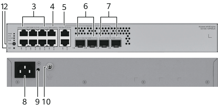
Figure 4-32 S310S-10PN4JX appearance
