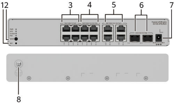
Figure 4-28 S310S-4P8UN2X appearance
