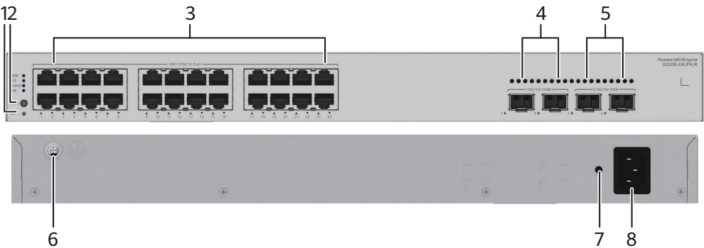
Figure 4-20 S220S-24LP4JX appearance
