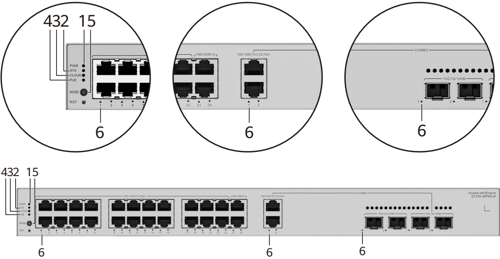
Figure 4-33 Indicators on the Switch
