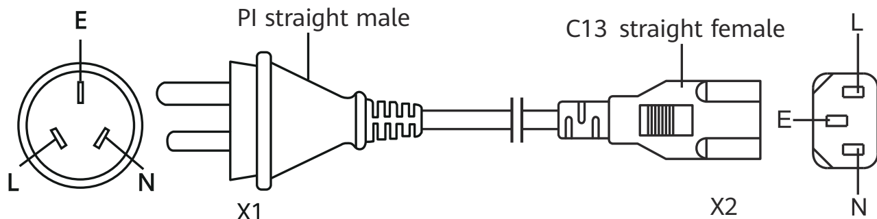
Figure 5-14 Structure of a PI straight male to C13 straight female AC power cable (used in China)
