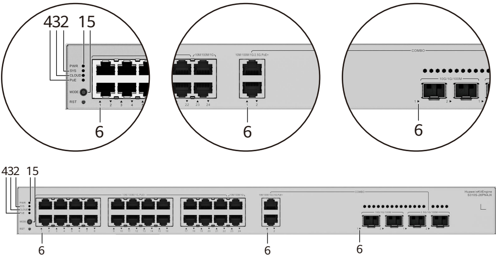
Figure 4-43 Indicators on the Switch
