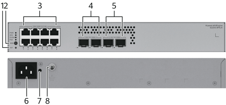
Figure 4-8 S220S-8P4JX appearance
