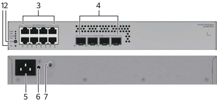
Figure 4-6 S220S-8P4J appearance
