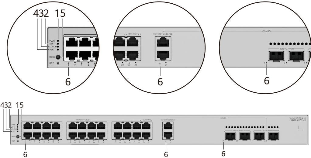
Figure 4-23 Indicators on the Switch
