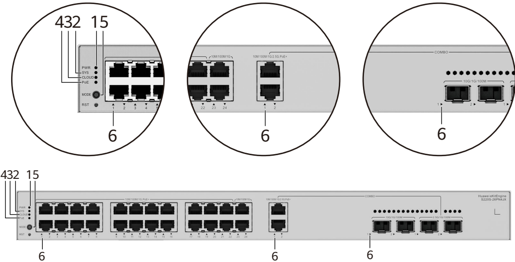
Figure 4-19 Indicators on the Switch
