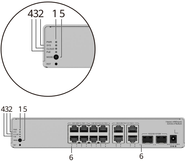
Figure 4-29 Indicators on the Switch
