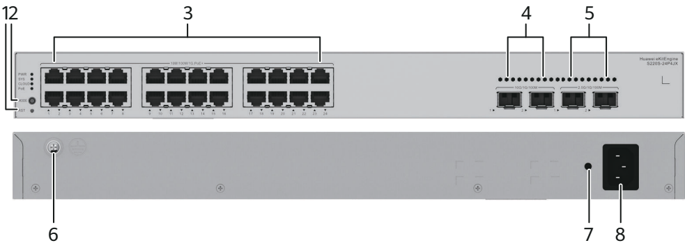
Figure 4-18 S220S-24P4JX appearance
