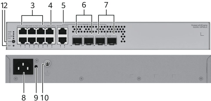
Figure 4-10 S220S-10PN4JX appearance
