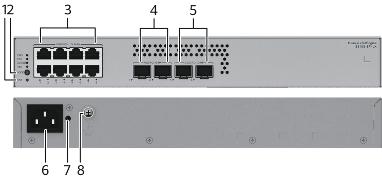
Figure 4-26 S310S-8P4JX appearance
