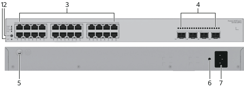
Figure 4-38 S310S-24P4J appearance
