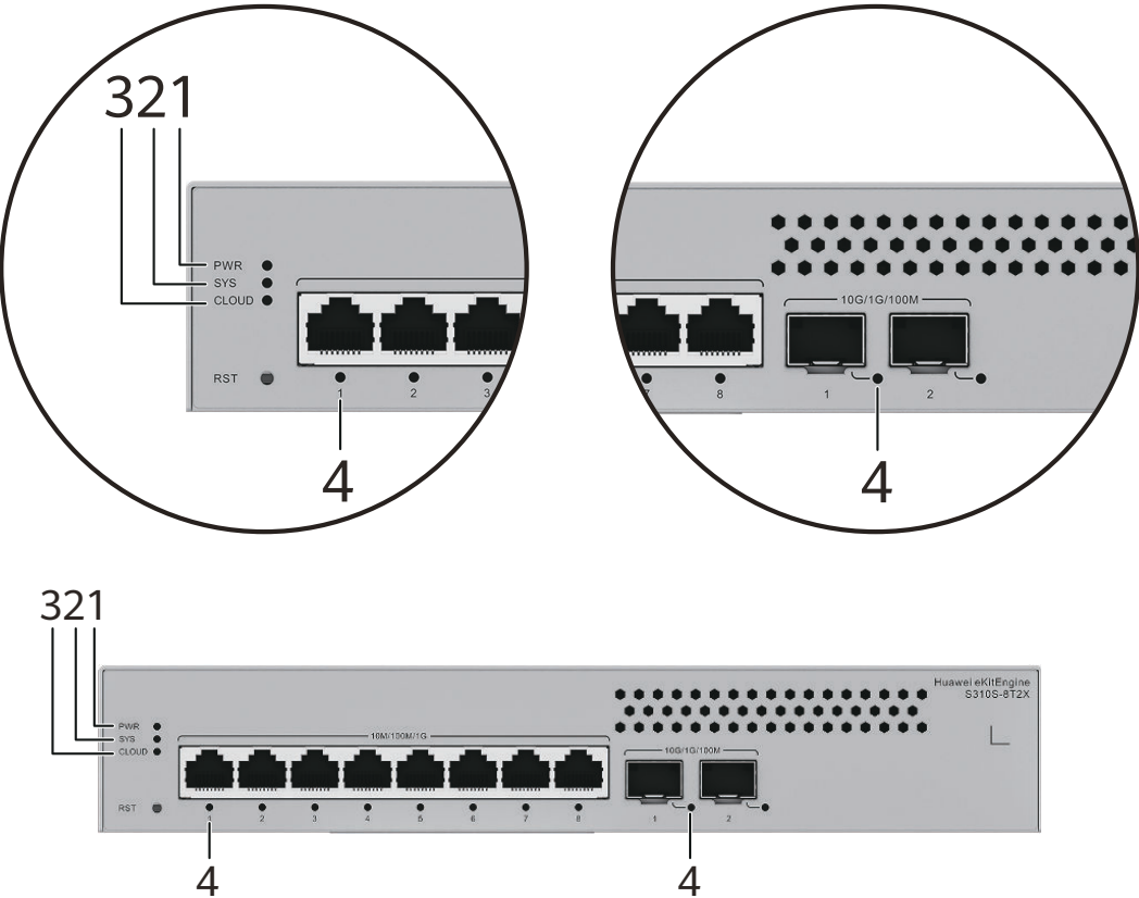
Figure 4-35 Indicators on the Switch
