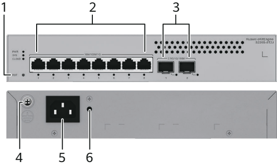
Figure 4-2 S220S-8T2J appearance
