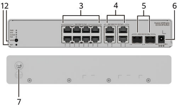
Figure 4-30 S310S-8P4UN2X appearance
