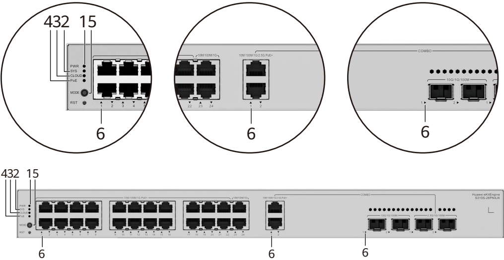
Figure 4-41 Indicators on the Switch
