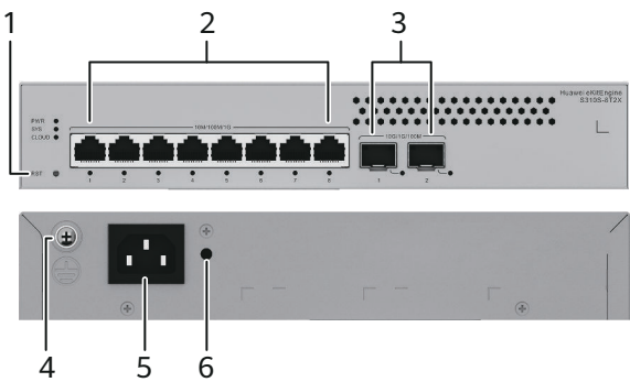
Figure 4-24 S310S-8T2X appearance
