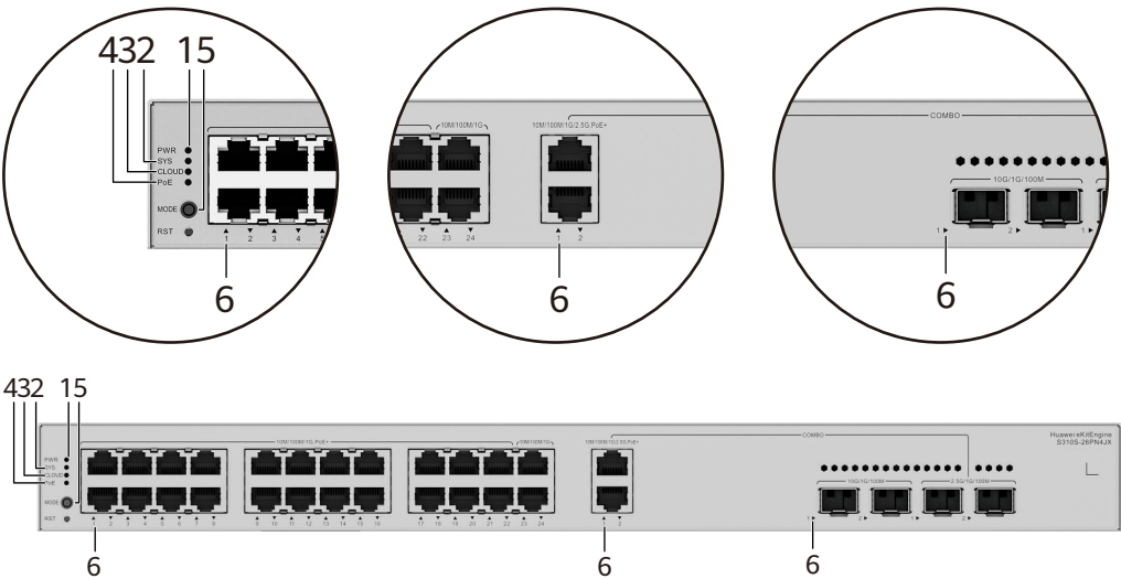
Figure 4-39 Indicators on the Switch
