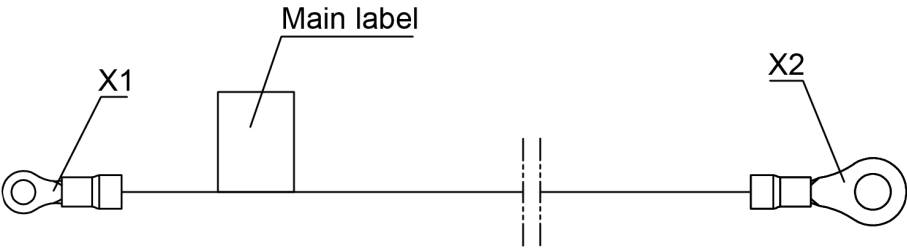
Figure 5-2 Structure of a ground cable
