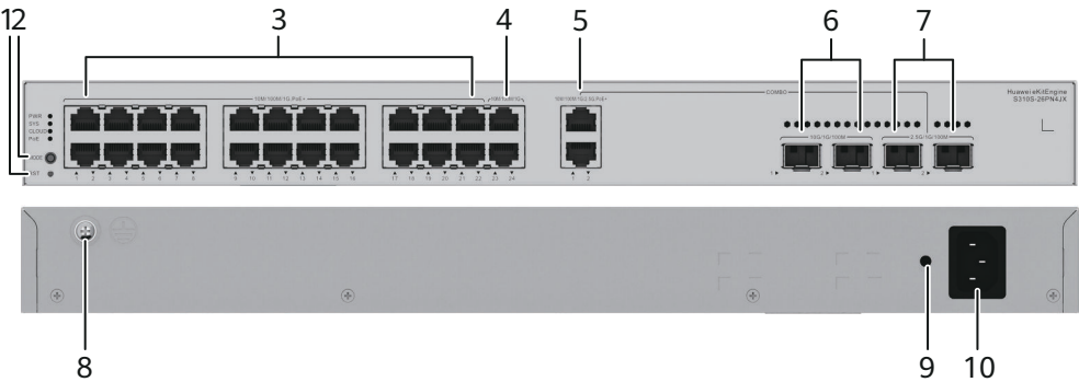
Figure 4-42 S310S-26PN4JX appearance
