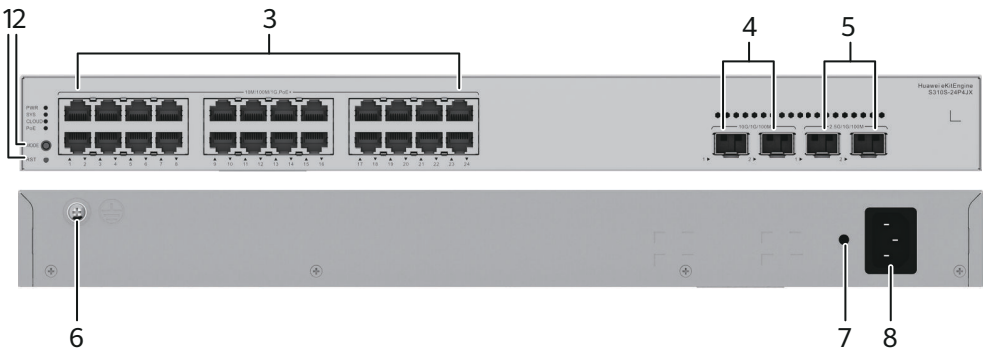
Figure 4-40 S310S-24P4JX appearance
