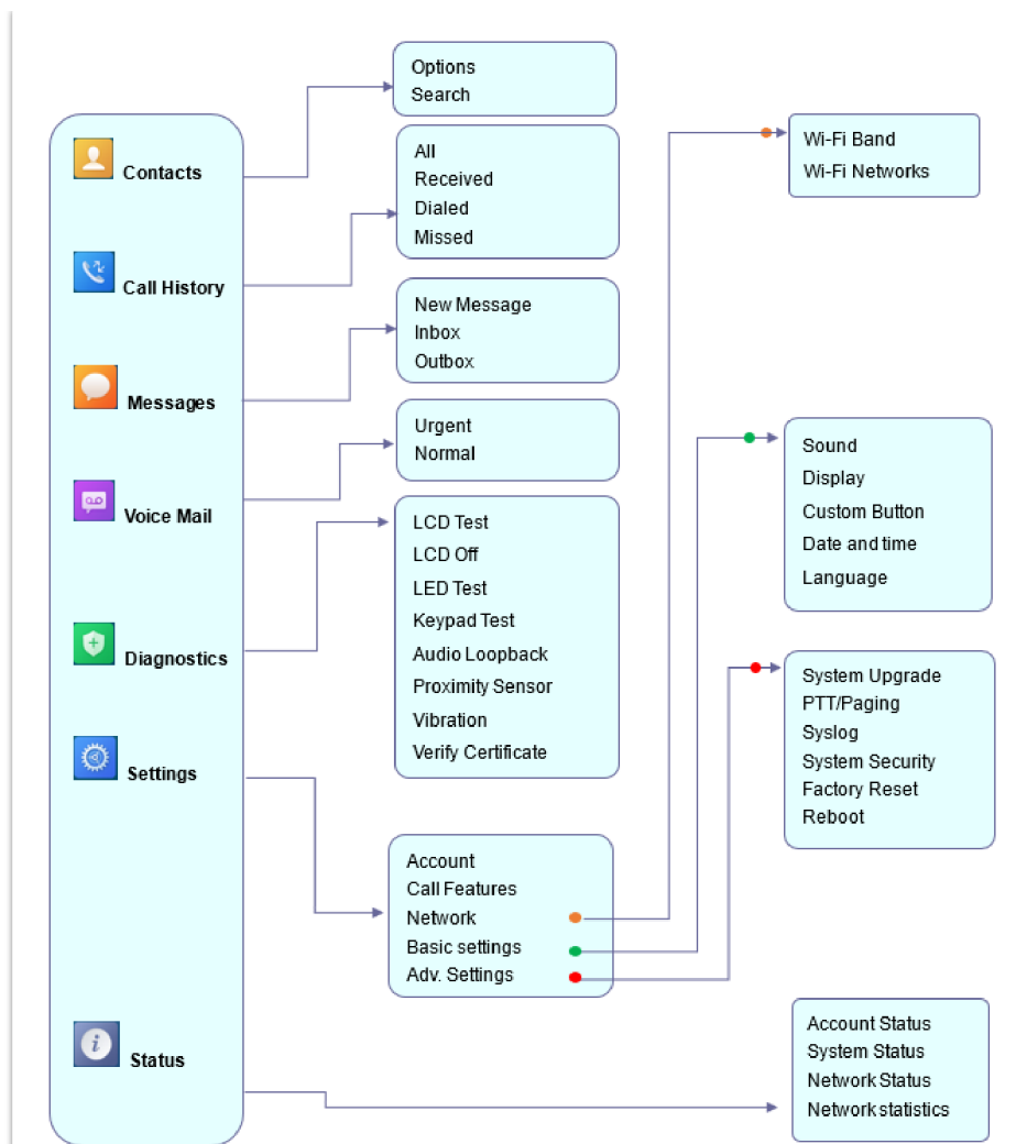
Menu Structure
