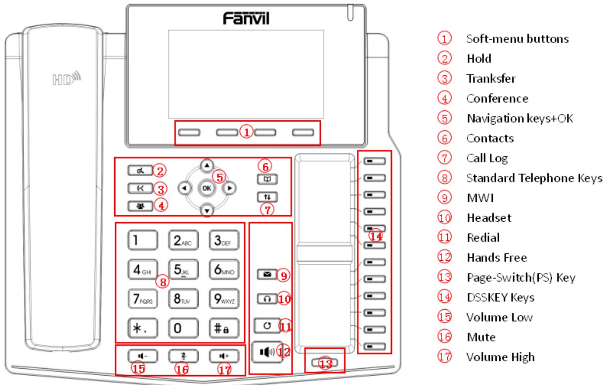
Figure 5 - Keypad
