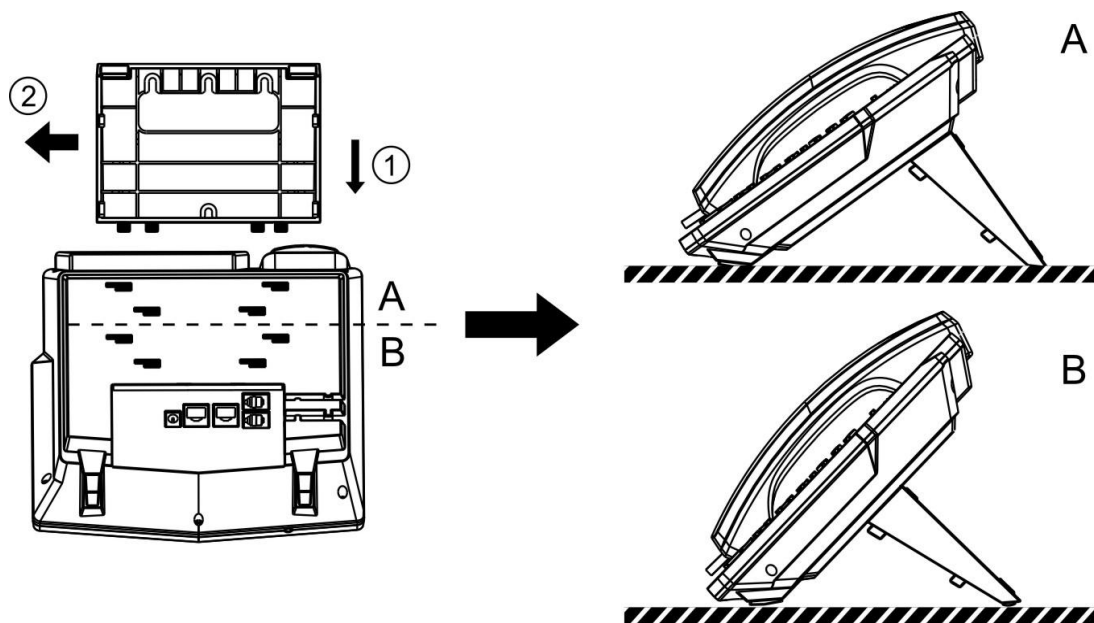
Figure 1 - Desktop Installation
